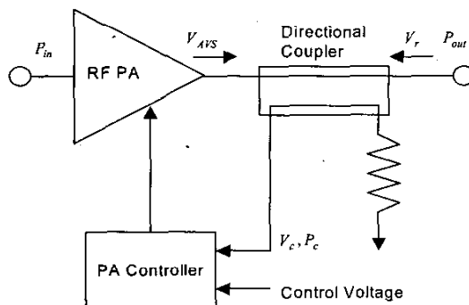
Fig. 1. PAM with integrated directional coupler and power control.
