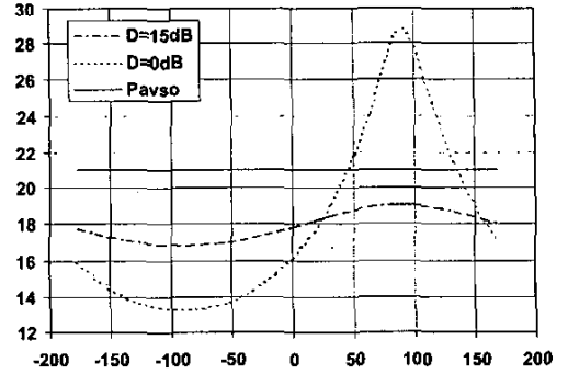
Fig. 3. Delivered power over phase when directivity is 15dB and 0dB as predicted by Eq. 6.
