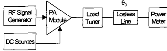
Fig. 5. Simplified block diagram of the load-pull setup.
